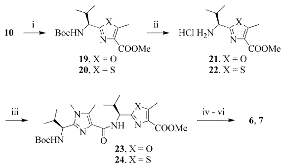
Scheme 4. i) \text{PPh}_3 , \text{Et}_3\text{N} , \text{CCl}_4 , 86% for 19 ; Lawesson's reagent, 75% for 20 . ii) \text{HCl}/\text{EtOAc} , quant. iii) 12 , DPPA, i\text{-Pr}_2\text{NEt} , 65% for 23 , 60% for 24 . iv) 2\text{ M NaOH} . v) \text{HCl}/\text{EtOAc} . vi) FDPP, i\text{-Pr}_2\text{NEt} , \text{CH}_3\text{CN} , 35% for 6 , 56% for 7 .
