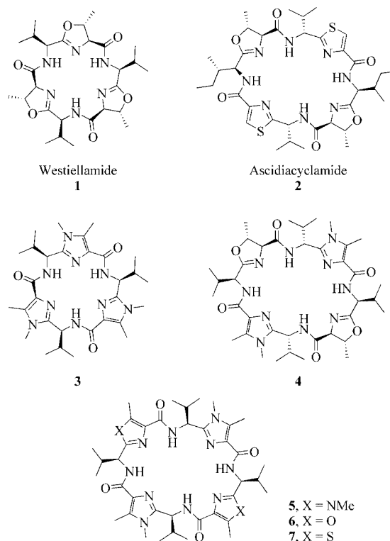
Figure 1. Lissoclinum cyclopeptides and their imidazole analogues
